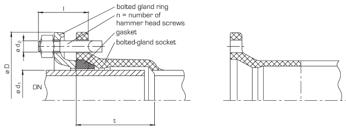
Socket for pipes and fittings
