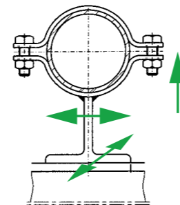
Fig. 4 loose support
